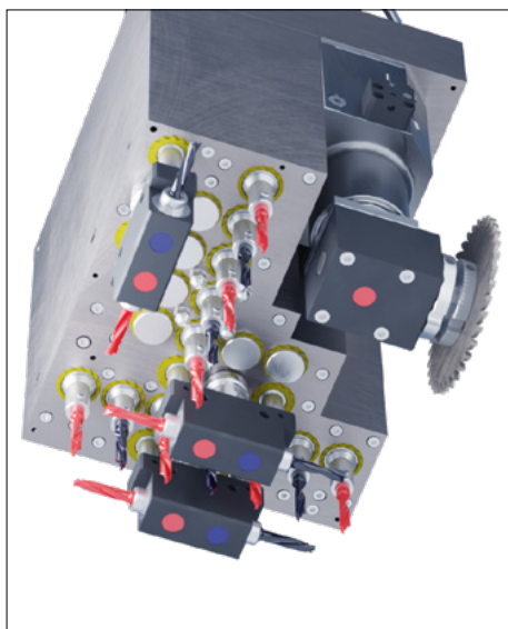
Konfiguration 18-Spindler
