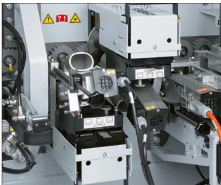
Fräsaggregat
