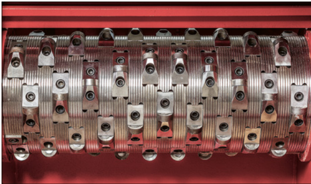
Rotor Version 5 (40 mm Messer-Ø)
