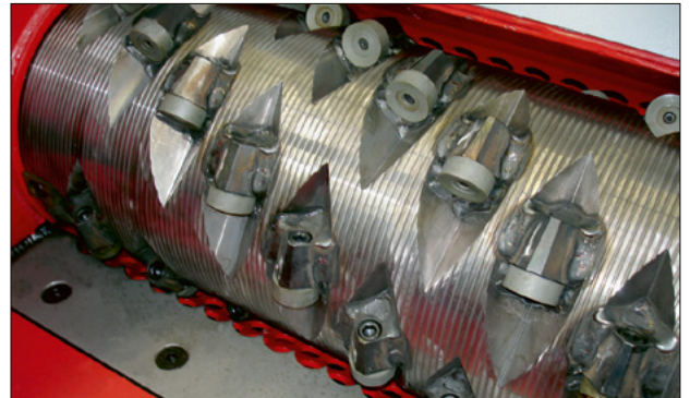
Rotor Version 7 (40 mm Messer-Ø)
