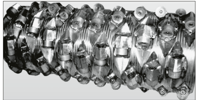
Rotor Version 8 (30 mm Messer-Ø)
