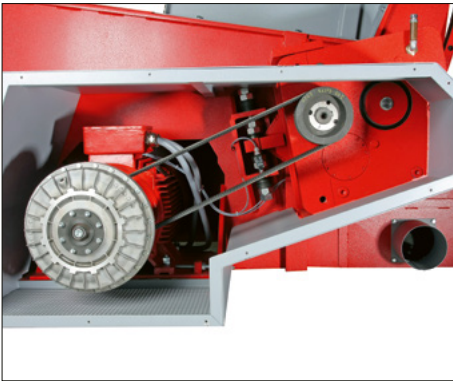
Turbo-Hydraulik ab 30 kW
